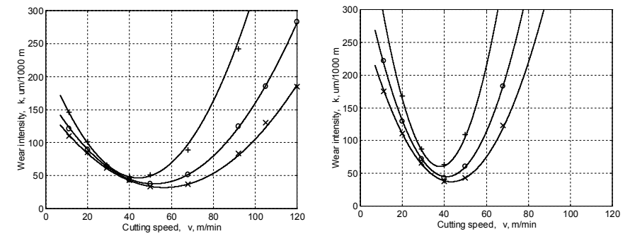
Figure 2 – Changing of wear intensity in function of cutting speed at different bore diameters +: d=45 mm; o: d=75 mm; x: d=100 mm (f=0.075 mm/rev.; a p =0.1 mm; VB=0.4 mm)
