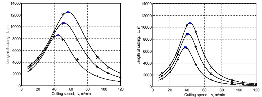
Figure 1 – The cutting length at different workpiece diameters +: d=45 mm; o: d=75 mm; x: d=100 mm (f=0.075 mm/rev.; a p =0.1 mm; VB=0.4 mm)
