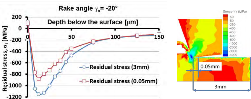
Figure 6 – The change depending on the depth of the surface layer ( \gamma_0 = -20^\circ )
