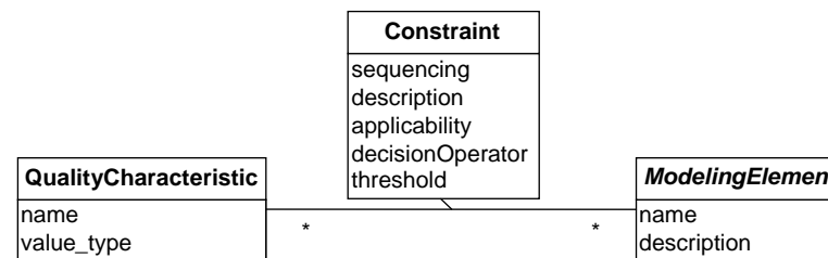
Figure 2: Part of QAPM metamodel describing the quality requirement as a constraint
