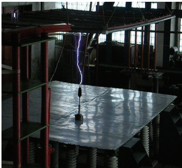
Figure 1 – General view of the test setup (air gap breakdown)
