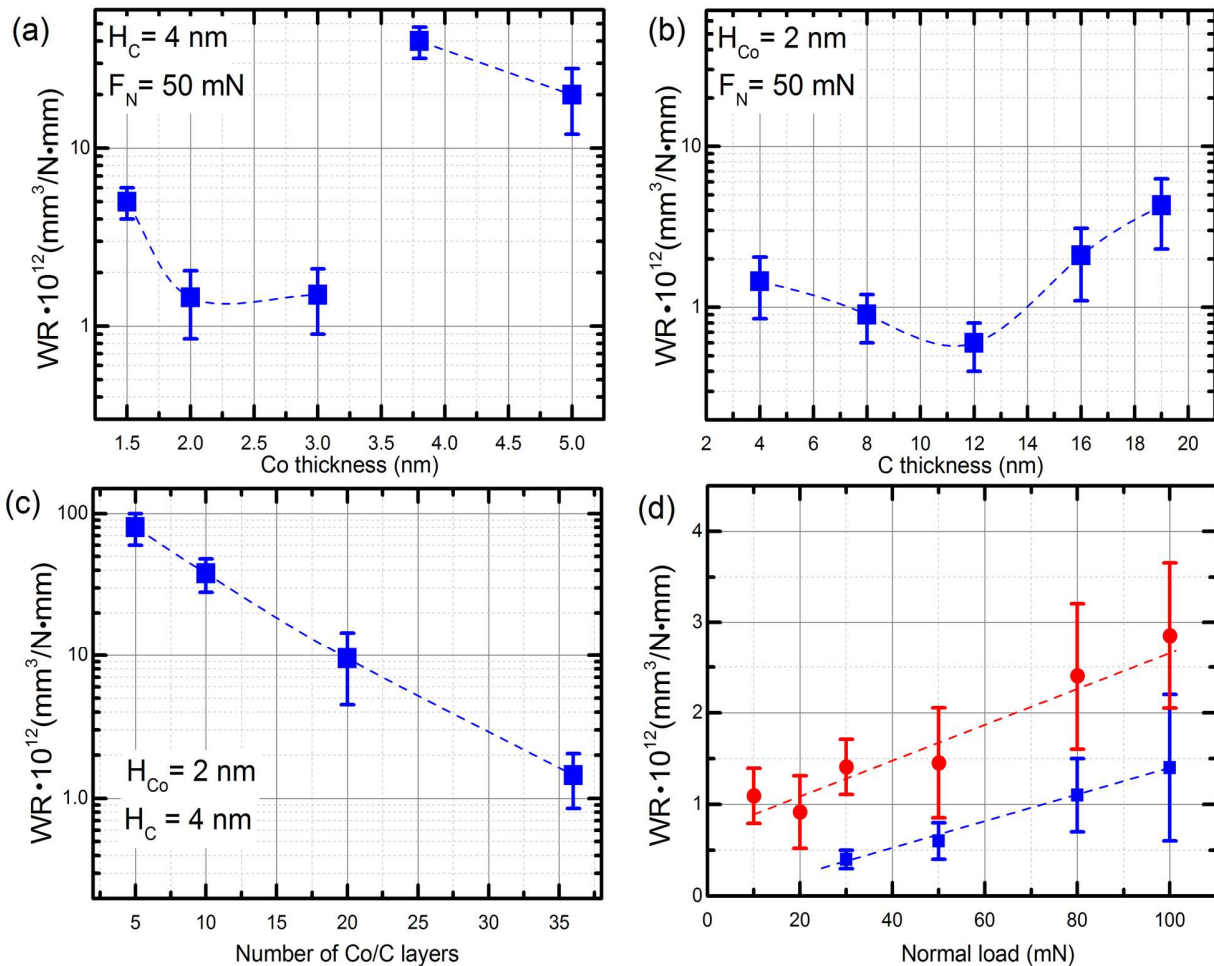
Figure 5. Wear behavior of Co/C PMCs. Wear rate as a function of (a) the thickness of the Co layers with the carbon thickness fixed at 4 nm and (b) the thickness of the carbon layers with the cobalt thickness fixed at 2 nm. (c) Wear rate as a function of the number of Co/C layers for the sample 2/4. (d) Wear rate as a function of the normal load for the samples 2/4 (red circles) and 2/12 (blue squares).
