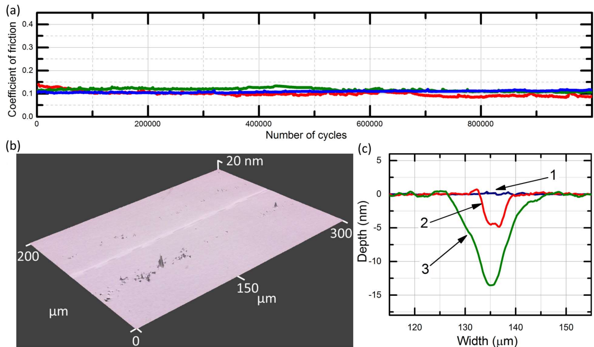
Figure 4. Friction and wear behavior of Co/C PMCs. (a) Friction coefficient as function of the sliding distance for three different tests and (b) 3D image of the wear track after 1 million sliding cycles under a load of 20 mN for the sample 2/12. (c) Variation in the profile of the wear track for various samples after 400,000 sliding cycles under a load of 20 mN: 1 – 2/12; 2 – 2/4; 3 – 3.8/4.
