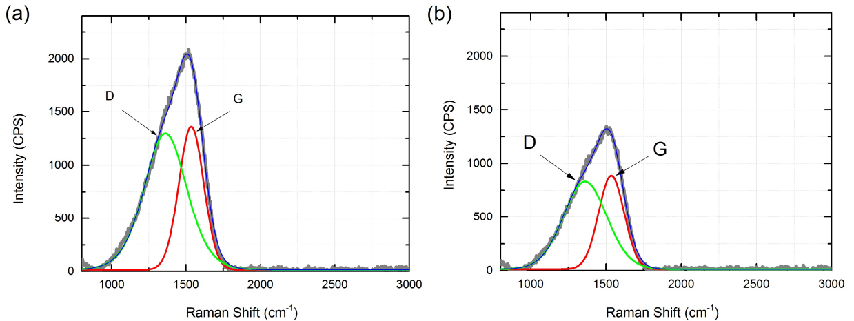
Figure 2. Raman spectroscopy data. D and G peaks of carbon for excitation wavelength of 532 nm for (a) 220 nm thick single layer carbon coating and (b) PMC 2/12.
