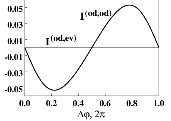
FIG. 2: The parts of the pumped currents which are odd in magnetic flux I_L^{(od,ev)} and I_L^{(od,od)} , Eqs.(34d) and (34e), are given as a function of the phase difference \Delta\varphi = \varphi^R - \varphi^L between the oscillating coupling parameters \epsilon^R(t) and \epsilon^L(t) for symmetric coupling: Both the left and the right wave splitters are coupled symmetrically to the branches of the ring. The currents are in units of e\omega/(2\pi) . The parameters are: L_1 = \pi ; L_2 = 0.7\pi ; \Phi = 0.4\Phi_0 ; \mu_0 = 9 ; V = 0.5 ; T_L = T_R = 0.1 ; \epsilon_0^L = \epsilon_0^R = 0.5 ; \epsilon_1^L = \epsilon_1^R = 0.4 . We use the following units: 2m_e = 1 ; \hbar = 1 ; e = 1 ; k_B = 1 .
