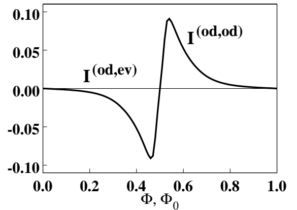
FIG. 3: The currents I_L^{(od,ev)} and I_L^{(od,od)} [in units of e\omega/(2\pi) ] as a function of the enclosed magnetic flux \Phi [in units of the magnetic flux quantum \Phi_0 = h/e ] for the case of symmetric coupling: Both the left and the right wave splitters are coupled symmetrically to the branches of a ring. The parameters are the same as in Fig.2. The phase difference is: \Delta\varphi = \pi/2 .
