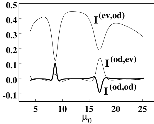
FIG. 4: The currents through the ring are given as a function of the Fermi energy \mu_0 . The coupling is asymmetric: Both the left and the right wave splitters are coupled asymmetrically to the branches of a ring. The parameters are the same as in Fig.2. The phase difference is: \Delta\varphi = \pi/2 . The currents I_L^{(od,ev)} and I_L^{(od,od)} are given in units of e\omega/(2\pi) . The current even in magnetic flux I_L^{(ev,od)} is given in dimensionless units of 1/(2\pi) .
