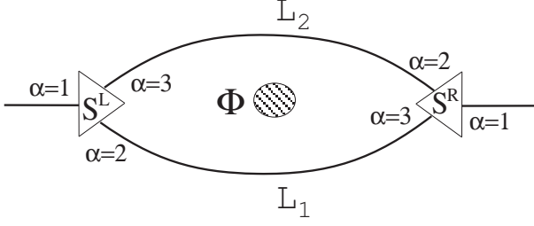
FIG. 1: A one-channel ring of length L = L_1 + L_2 with enclosed magnetic flux \Phi and with two leads. The Greek letter \alpha numbers the scattering channels at the left S^L and right S^R wave splitters.
