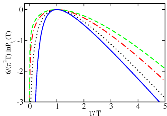
FIG. 2: Normalised logarithm of the probability distribution \mathcal{P}_{t_0}(T) as a function of T/\bar{T} , with \bar{T} the average value of T . The curves correspond to the narrow Gaussian wavepacket energy distribution (blue solid) in Eq. (16) and to an exponential energy distribution with \alpha = 1 (black dotted), 3 (red dash-dotted), 5 (green dashed). See text for details.
