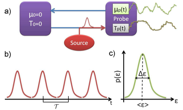
FIG. 1: a) Schematic of an on-demand source injecting single particle wavepackets into an electronic probe, via the lower edge state of a conductor in the quantum Hall regime. The probe is in the hot-electron regime, with a floating electron temperature T_p(t) and chemical potential \mu_p(t) . Particles emitted from the probe flow along the upper edge into an electronic reservoir electrically grounded and kept at zero temperature. b) Noiseless train of wavepackets, emitted from the single particle source with a frequency \omega = 2\pi/\mathcal{T} . c) Probability distribution of energy p(\epsilon) of the wavepacket, with average \langle \epsilon \rangle and width \Delta \epsilon shown.
