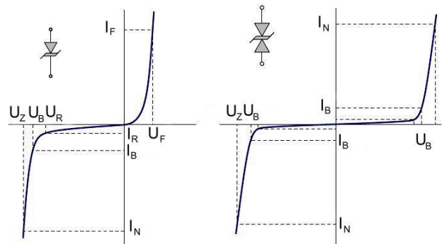
Fig. 20. Volt-amps diagram of mono-directional (DC) and bidirectional (AC) diode suppressors
