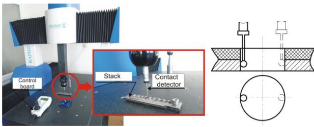
Fig. 4 – Schematic of measuring hole accuracy
