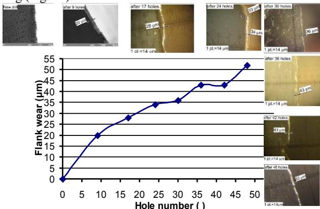
Fig. 11 – Progress of flank wear during CFRP/steel stack machining
