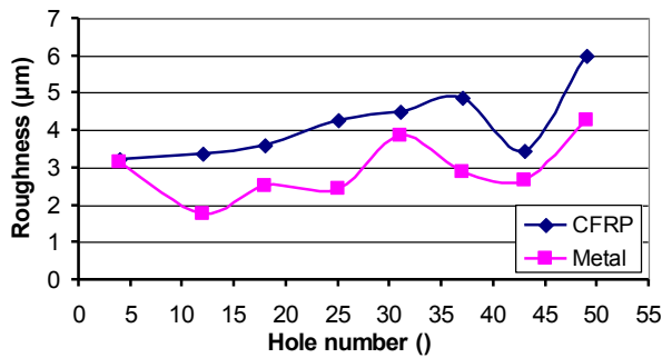
Fig. 10 - Hole roughness in CFRP and Steel part
