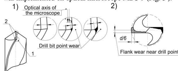
Fig.3 – Schematic of measuring flank wear of the drill on instrumental microscope
